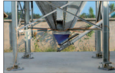
Electronic silo weighing
